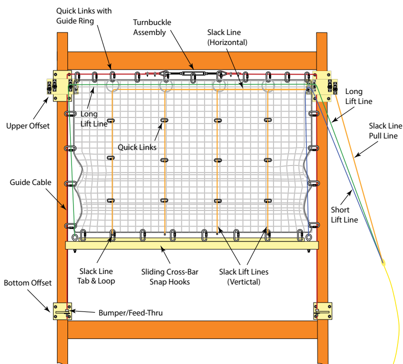
Shown Above: Drop to Close with Slack Limiter option.
